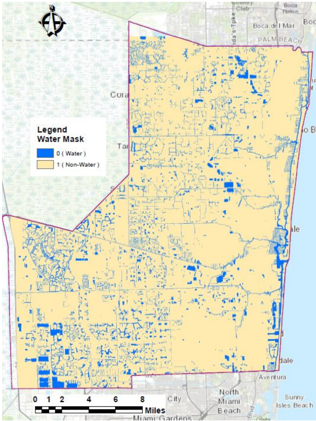
Figure 3-8 Water bodies
