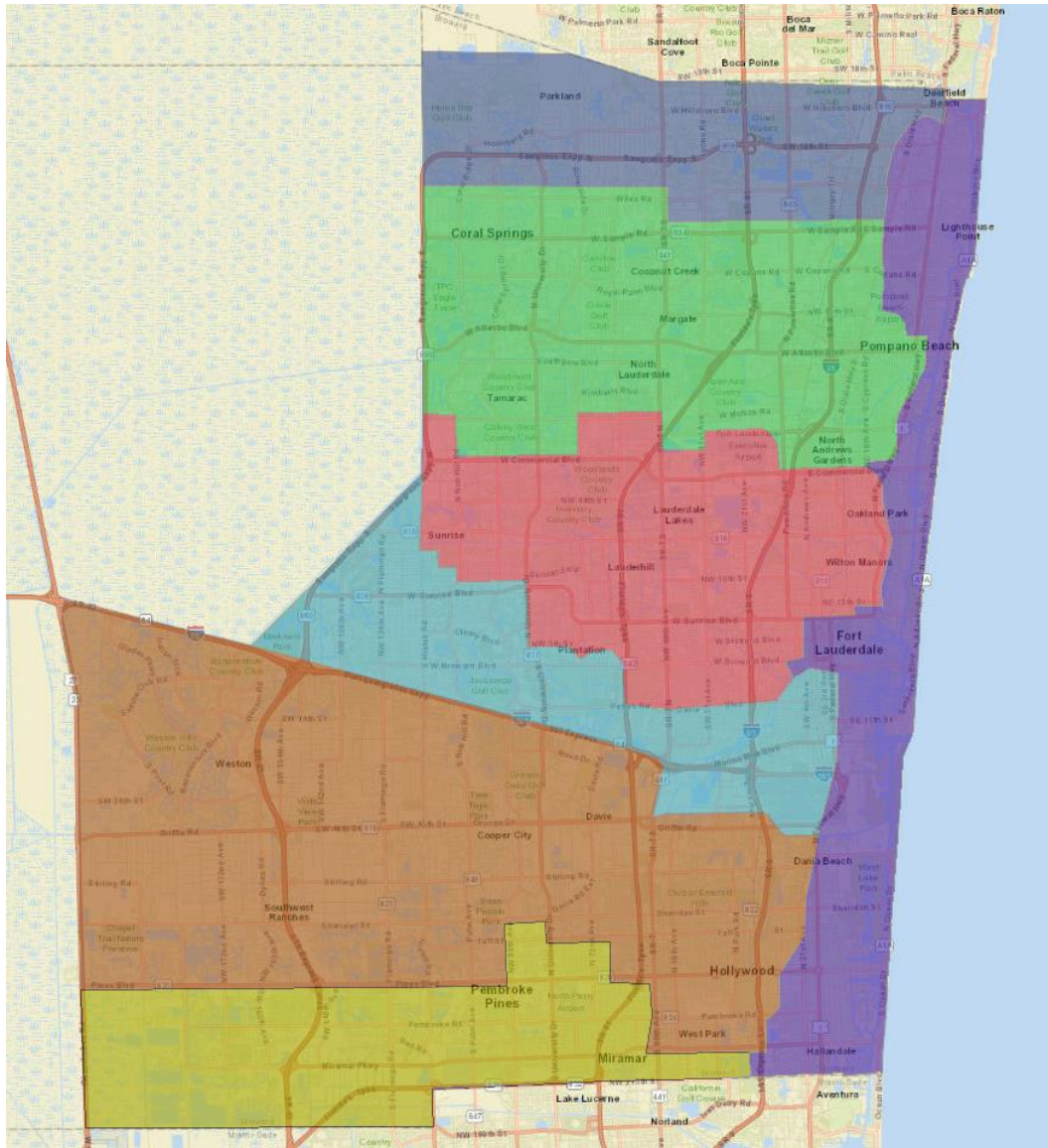
Figure 3-10 Broward County basins
