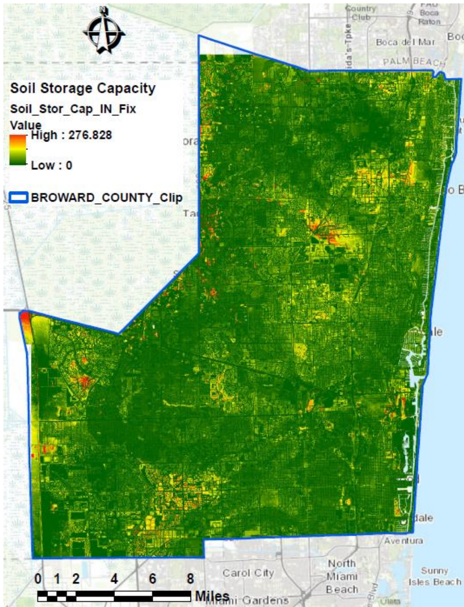
Figure 3-6 – Soil storage capacity
