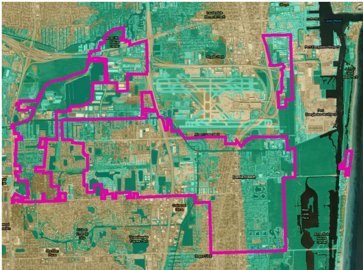
Figure 3-15 Projected Dania Beach flooding
