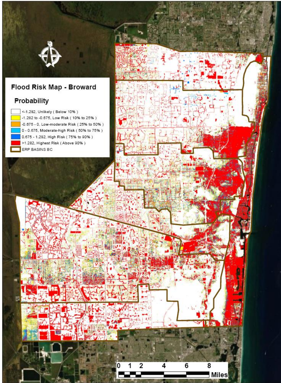
Figure 3.12 – Probability of Flooding for the 3 day 25 year storm event.
