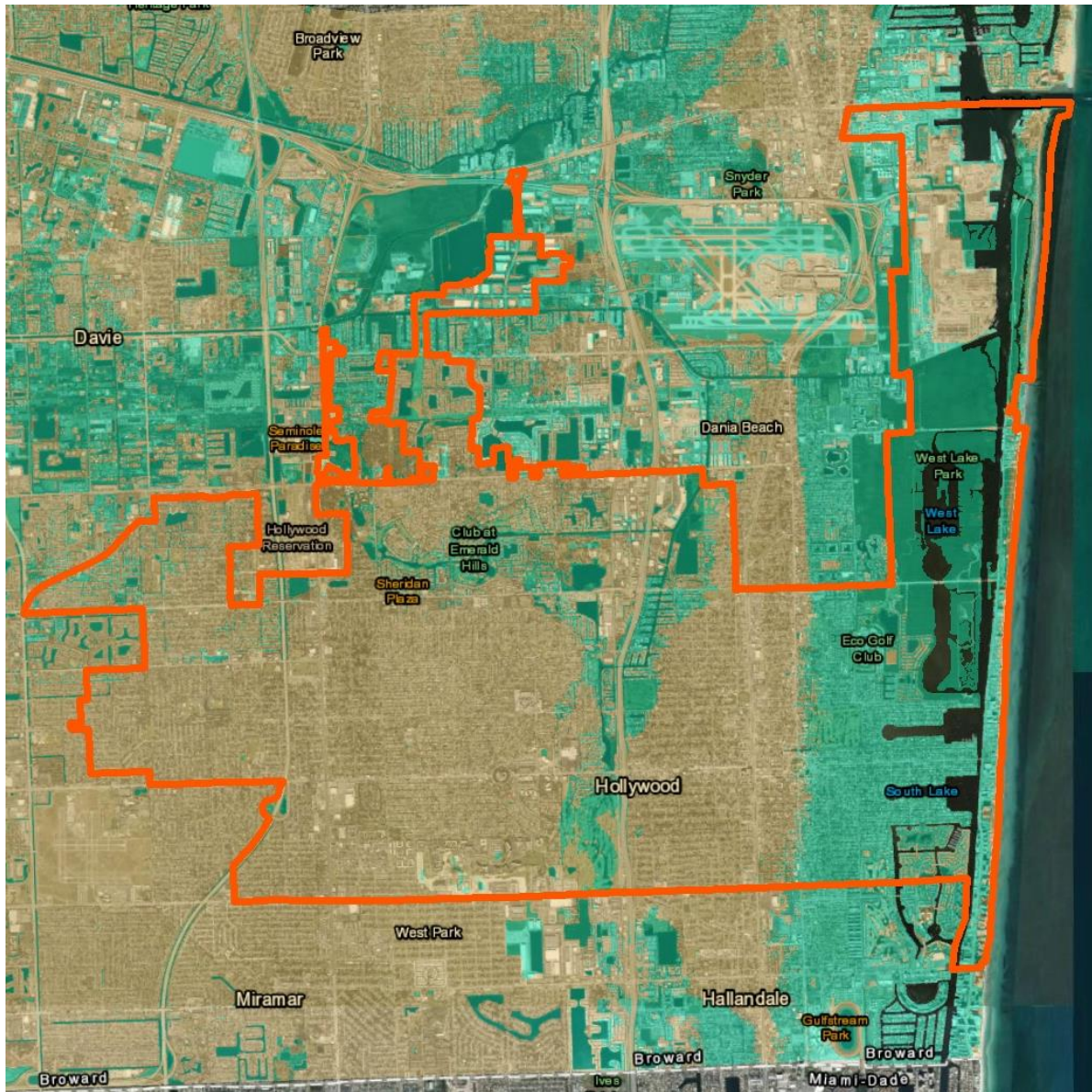
Figure 3-16 Projected Hollywood flooding
