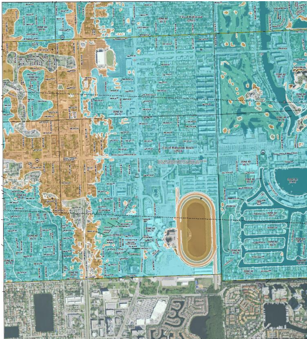
Figure 3-17 Projected Hallandale Beach flooding
