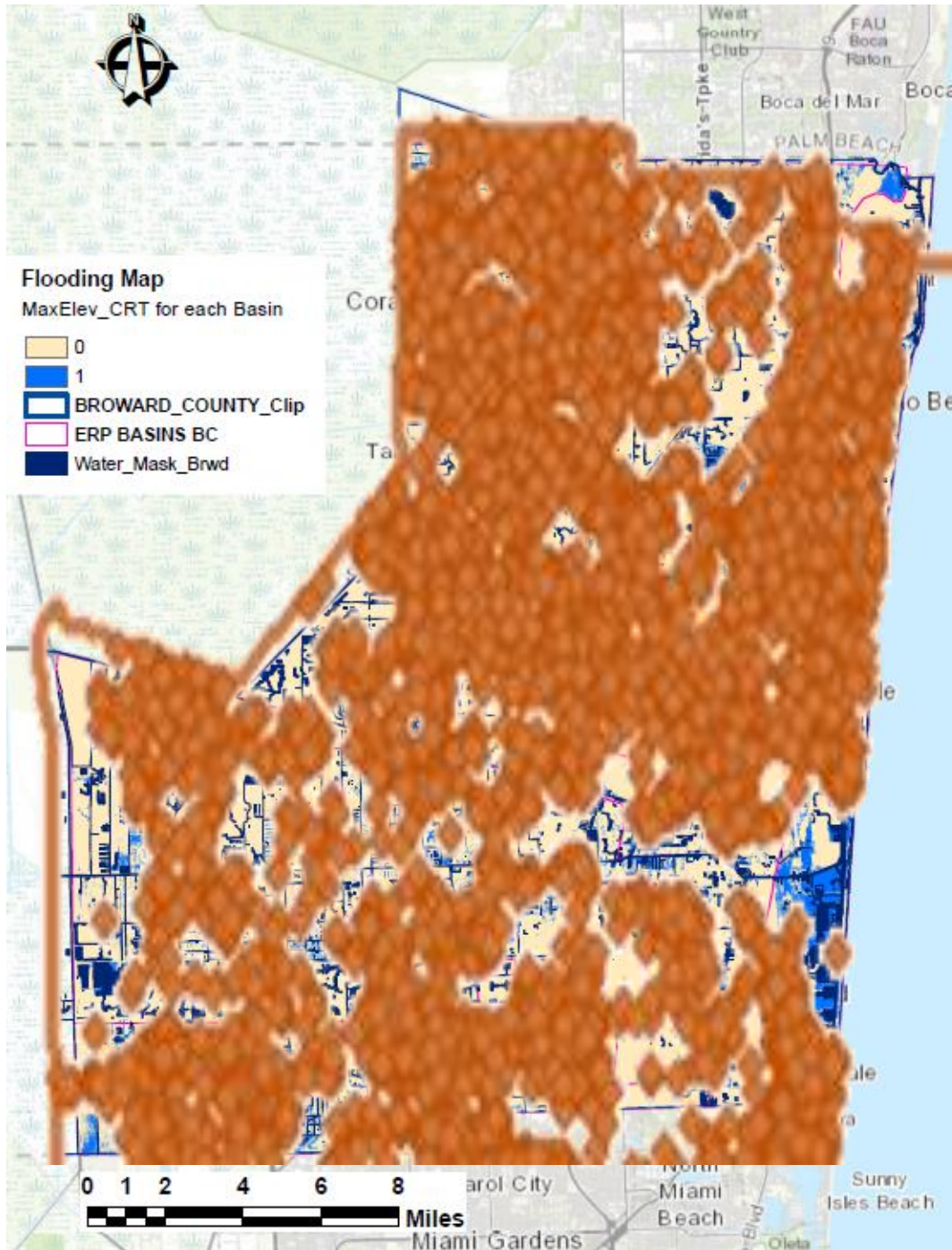
Figure 3.14 Repetitive loss areas from 2004 -2014 superimposed on the flood risk map created by FAU.
