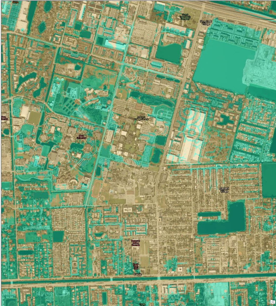
Figure 3-19 Projected Davie flooding
