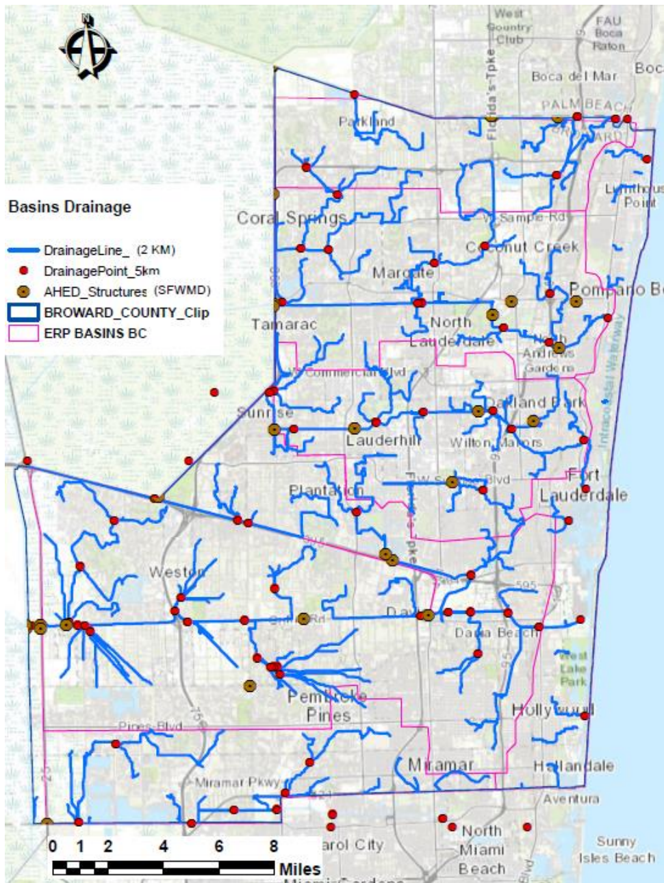
Figure 3-9 Broward County flow paths
