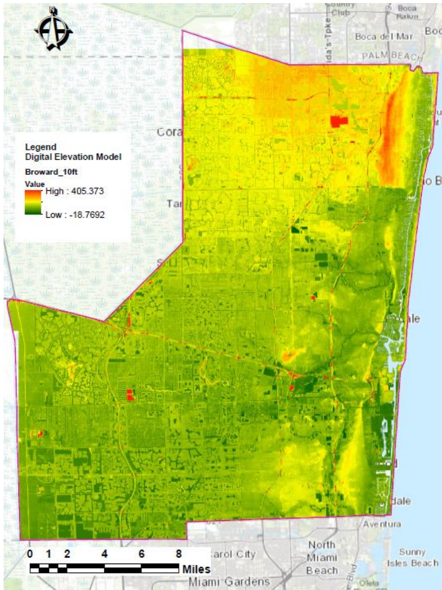
Figure 3.1 Topography of Broward County based on Lidar DEM
