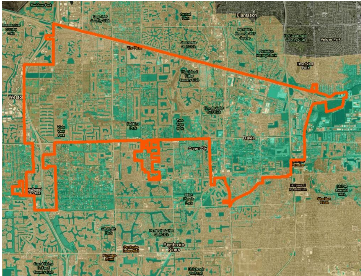
Figure 3-18 Projected Dania Beach flooding
