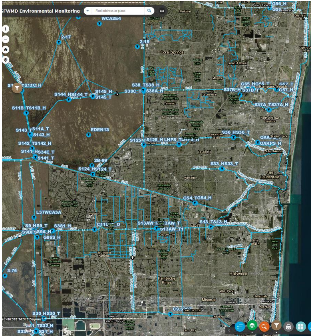
Figure 3.2 Water bodies and canals in Broward County
