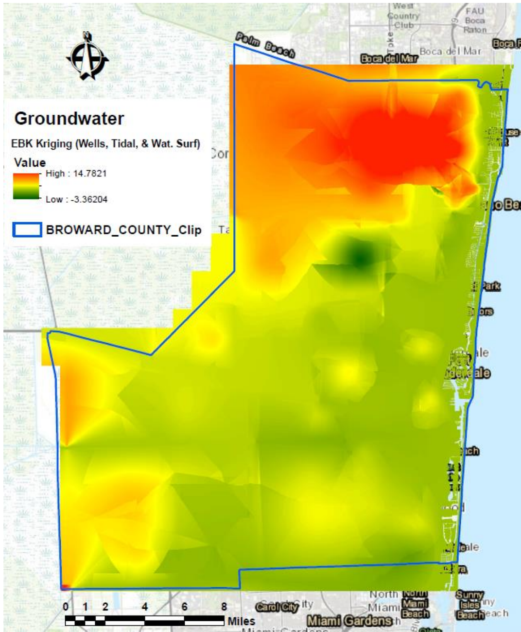
Figure 3-4 Groundwater layer
