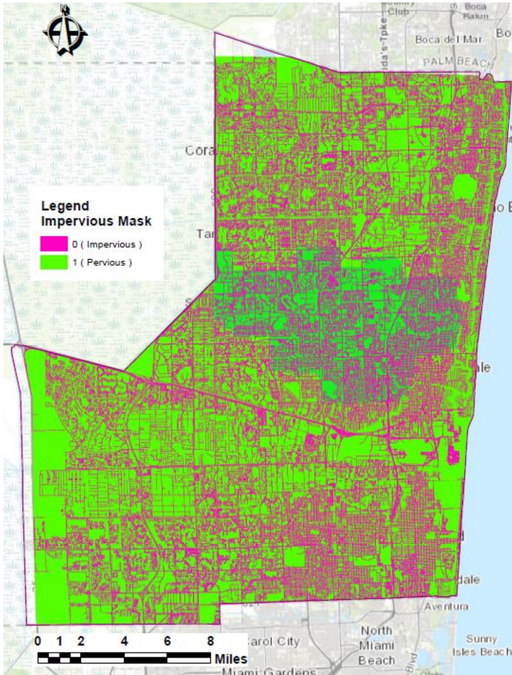
Figure 3-7 Impervious areas in Broward
