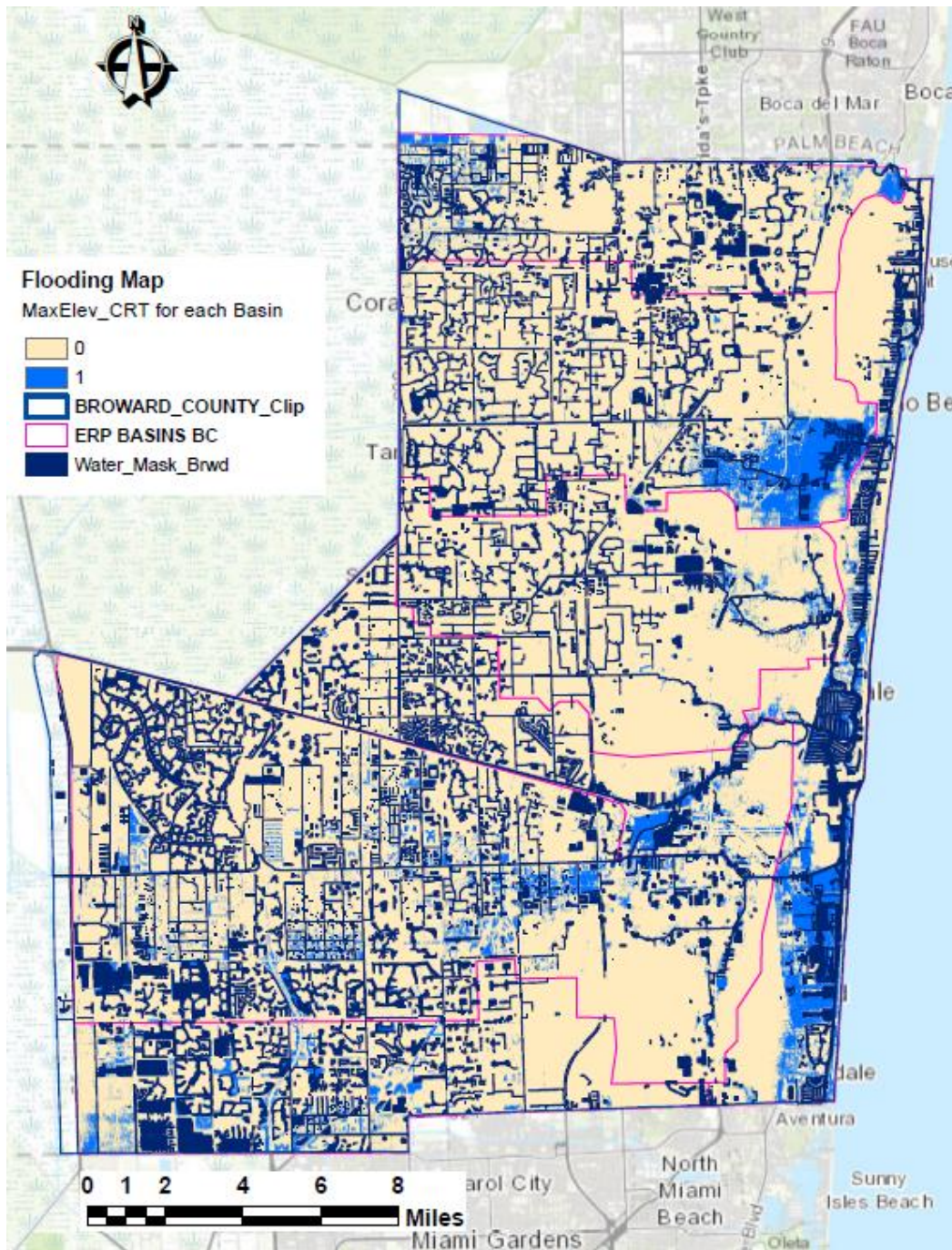
Figure 3-11 Flooding predicted based on the 3 day 25 year storm.
