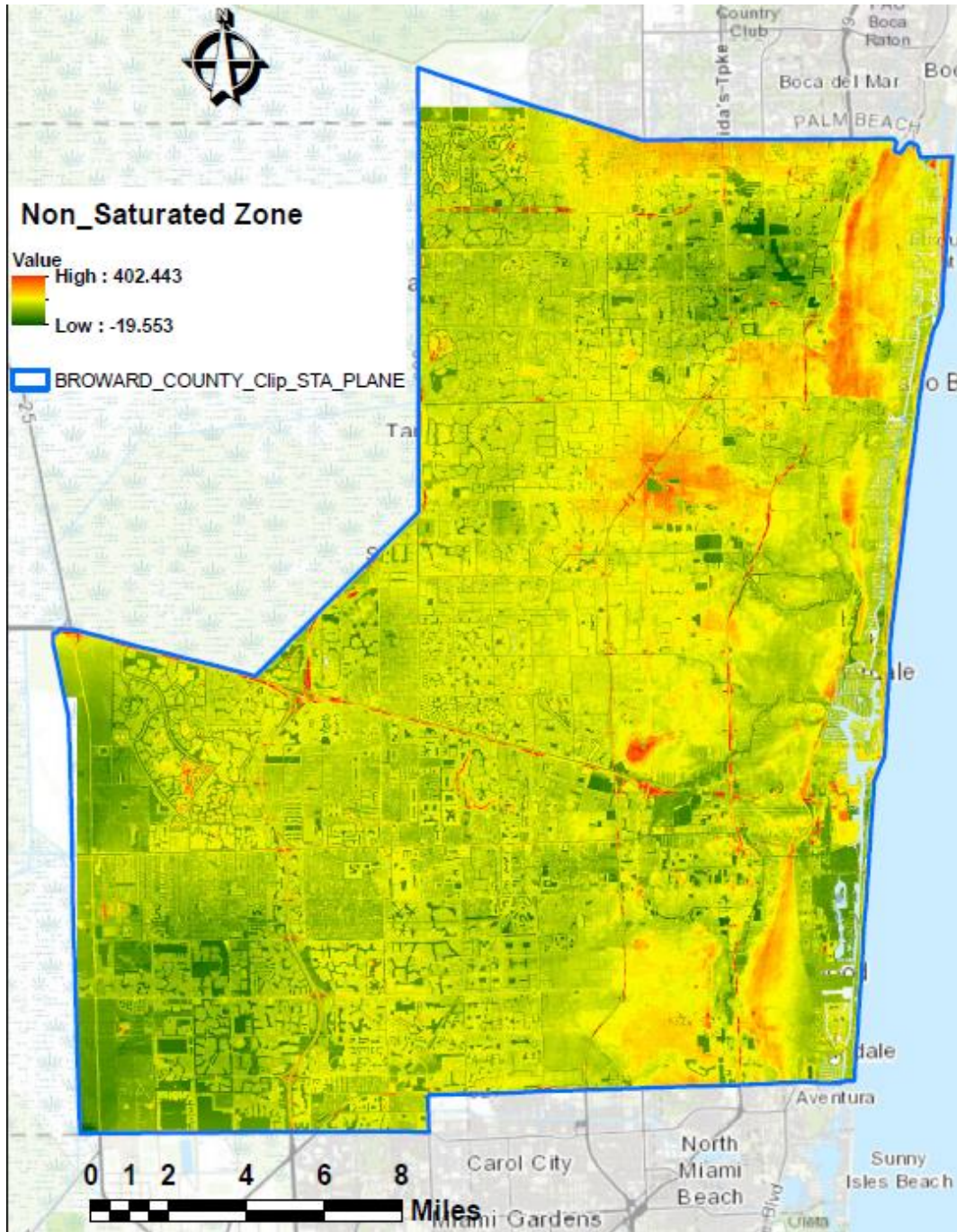
Figure 3-5 Unsaturated zone
