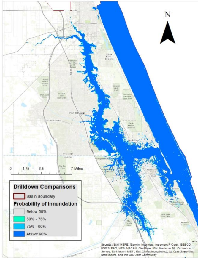
Figure 3.16: Drilldown study of Port St. Lucie
