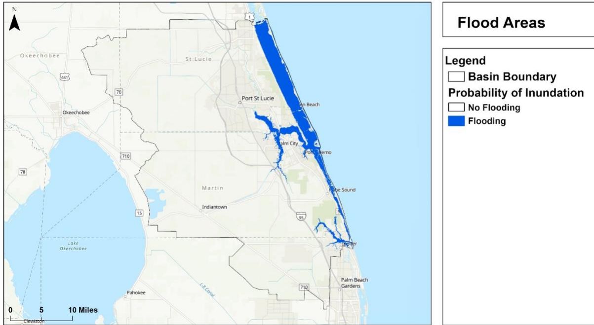
Figure 3.12: Flood risk map for St. Lucie- Loxahatchee
