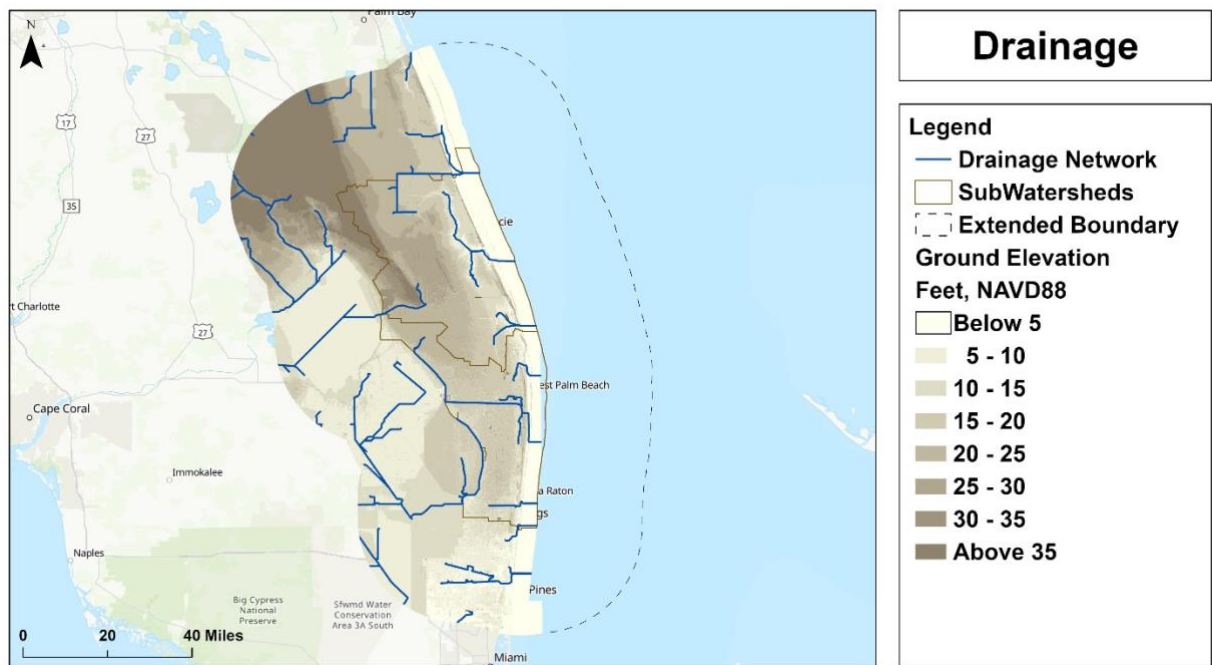
Figure 3.9: Drainage Network
