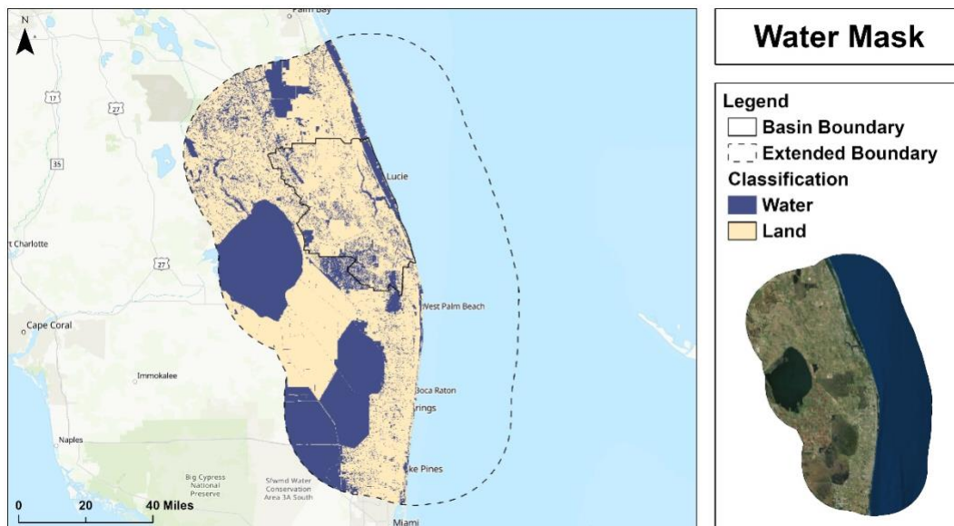
Figure 3.4: Water mask of the study area.
