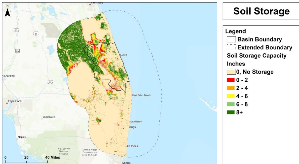
Figure 3.8: Soil Storage Capacity
