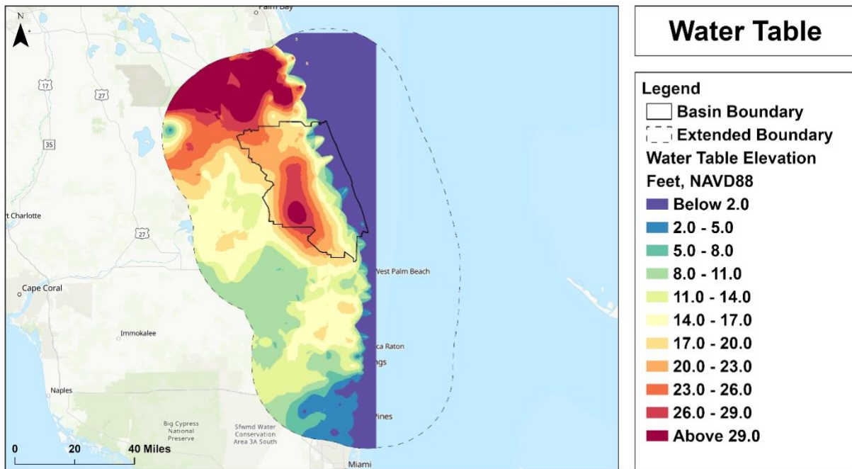
Figure 3.6: Water table Elevation
